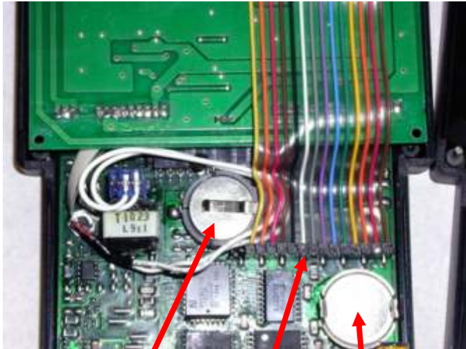
Renata CR1632 Battery (Our part # E0310 )
