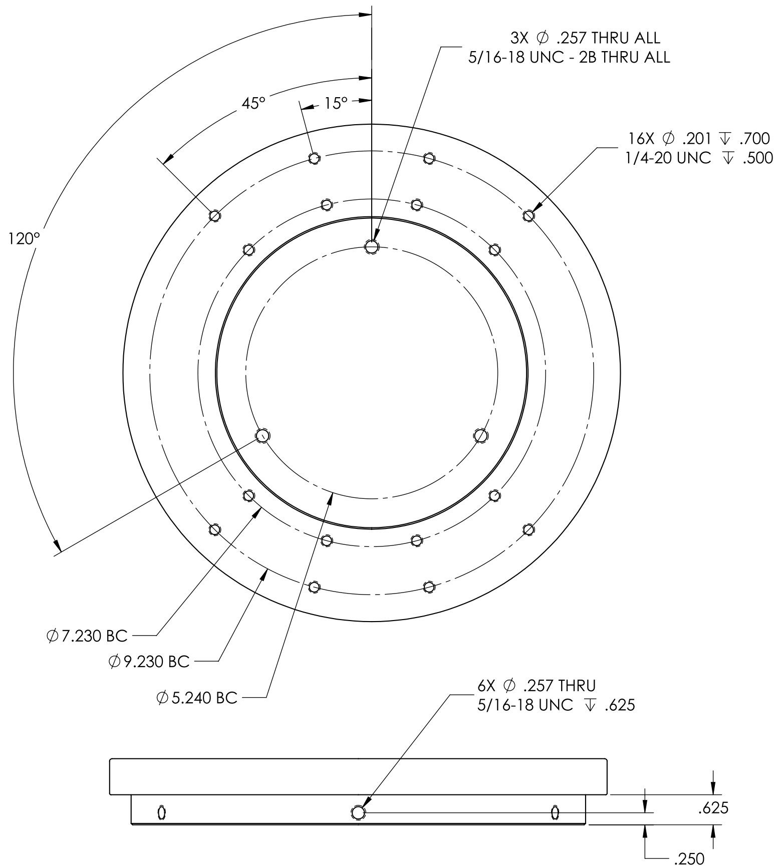
10" Flat Pier Plate (1612FP)
