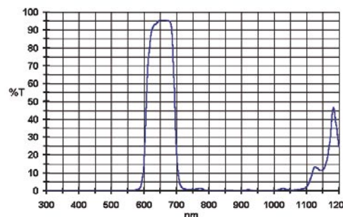
Spectral trace BAADER UV/IR-Cut Filter & BAADER RG 610 Red Color Filter, working as H-α pass-filter
